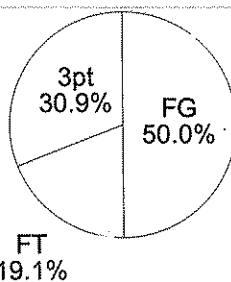
Scoring Distribution
